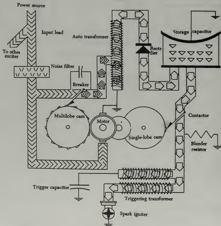
FIGURE 4-76. Capacitor-type ignition system schematic.
